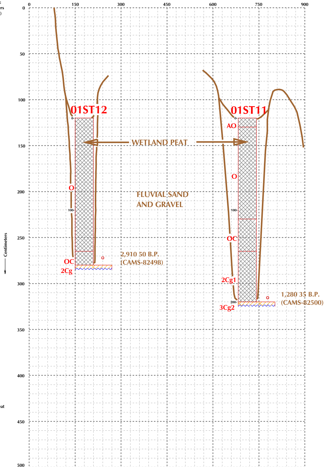
FIGURE 19 GRAPHIC SEDIMENT/ SOIL LOGS OF THE VT1MA LANDFORM SEDIMENT ASSEMBLAGE ALONG A TRANSECT CONTAINING CORES 01ST11-12
