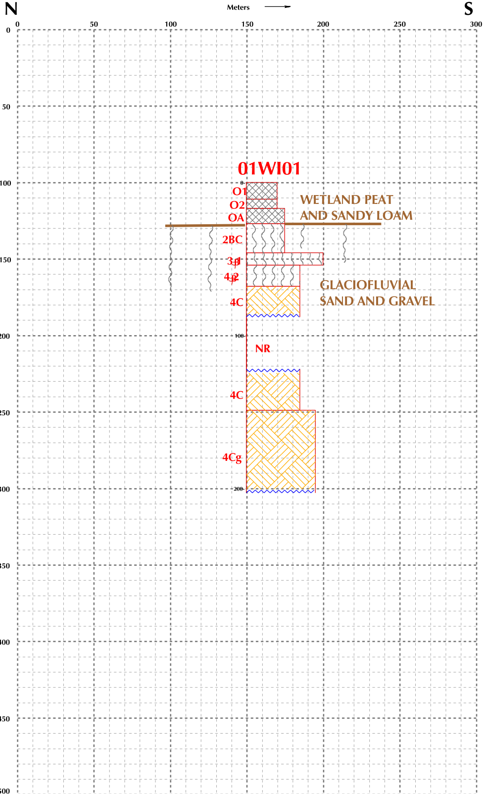
FIGURE 7B GRAPHIC SEDIMENT/ SOIL LOGS OF THE CPC LANDFORM SEDIMENT ASSEMBLAGE AT CORE LOCATIONS 01SH01 AND 01WI01
